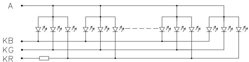
CIRCUIT DIAGRAM
